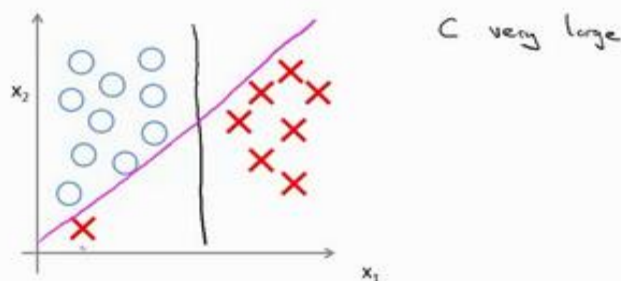
Large margin classifier in presence of outliers
